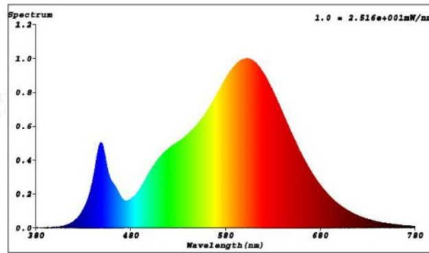
Spectral power distribution for FH-VVL-U-10VWV
